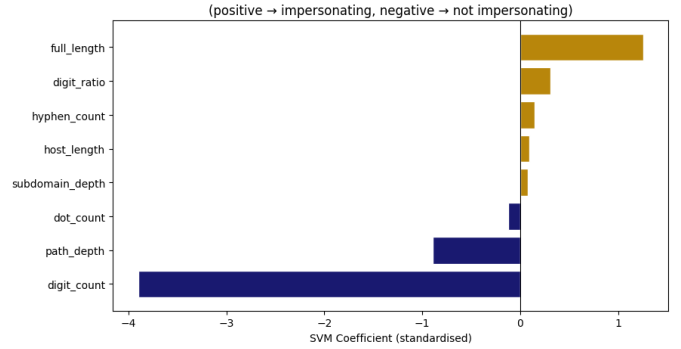
Fig. 7. Linear SVM Feature Coefficients
