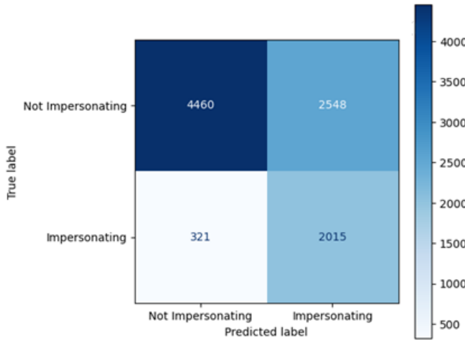
Fig. 4. Confusion Matrix for Tuned RBF SVM
