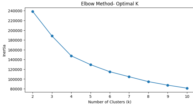
Fig. 6. Elbow Curve for Baseline Lexical Clustering
